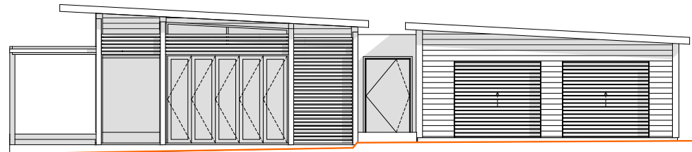
NORTH ELEVATION scale 1:150
